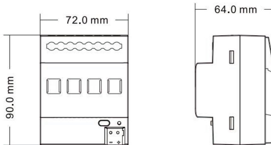
KNX-7043-82-DRO-DIN
