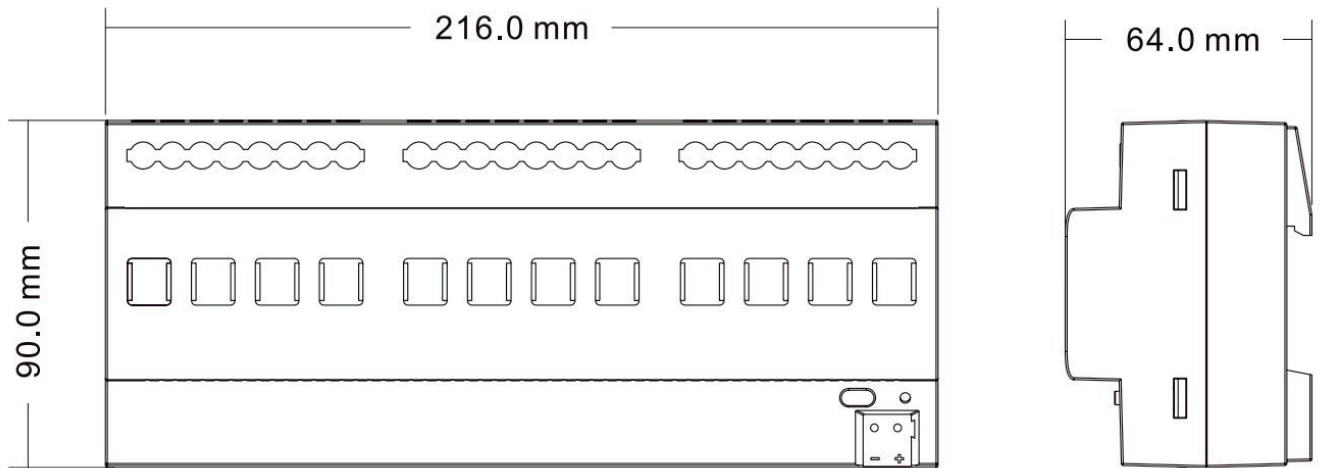
KNX-7123-82-DRO-DIN
